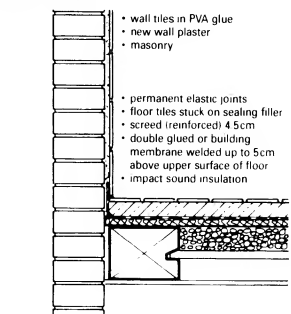
⑬ Floor/wall structure in damp areas in a masonry building with wooden beam floors
